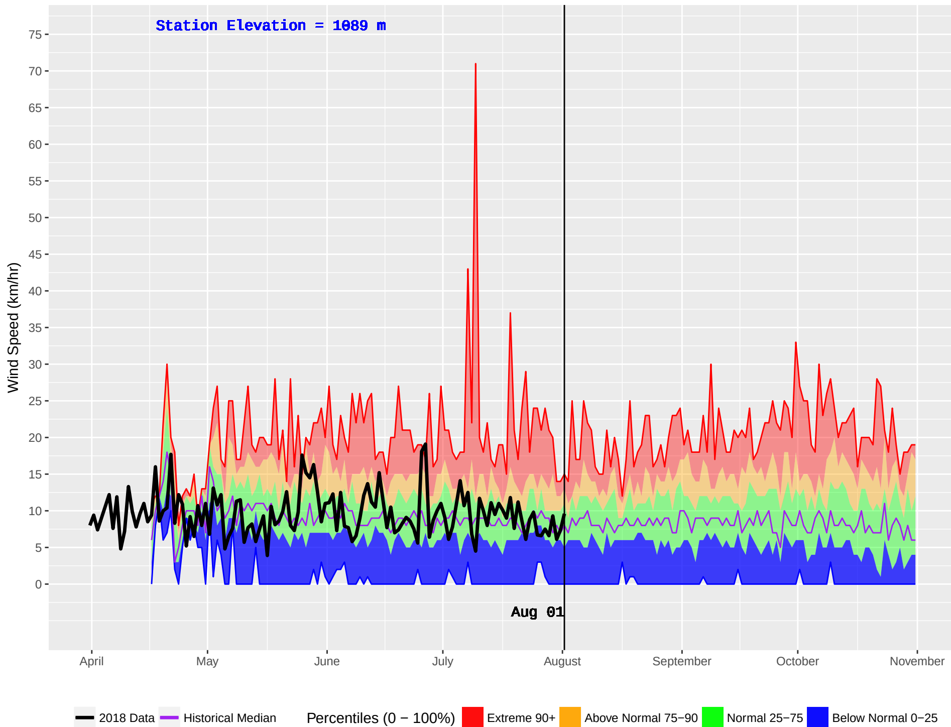
EAST OOTSA (170) : Historical (1986–2016) and Current (2018) Daily Wind Speed
