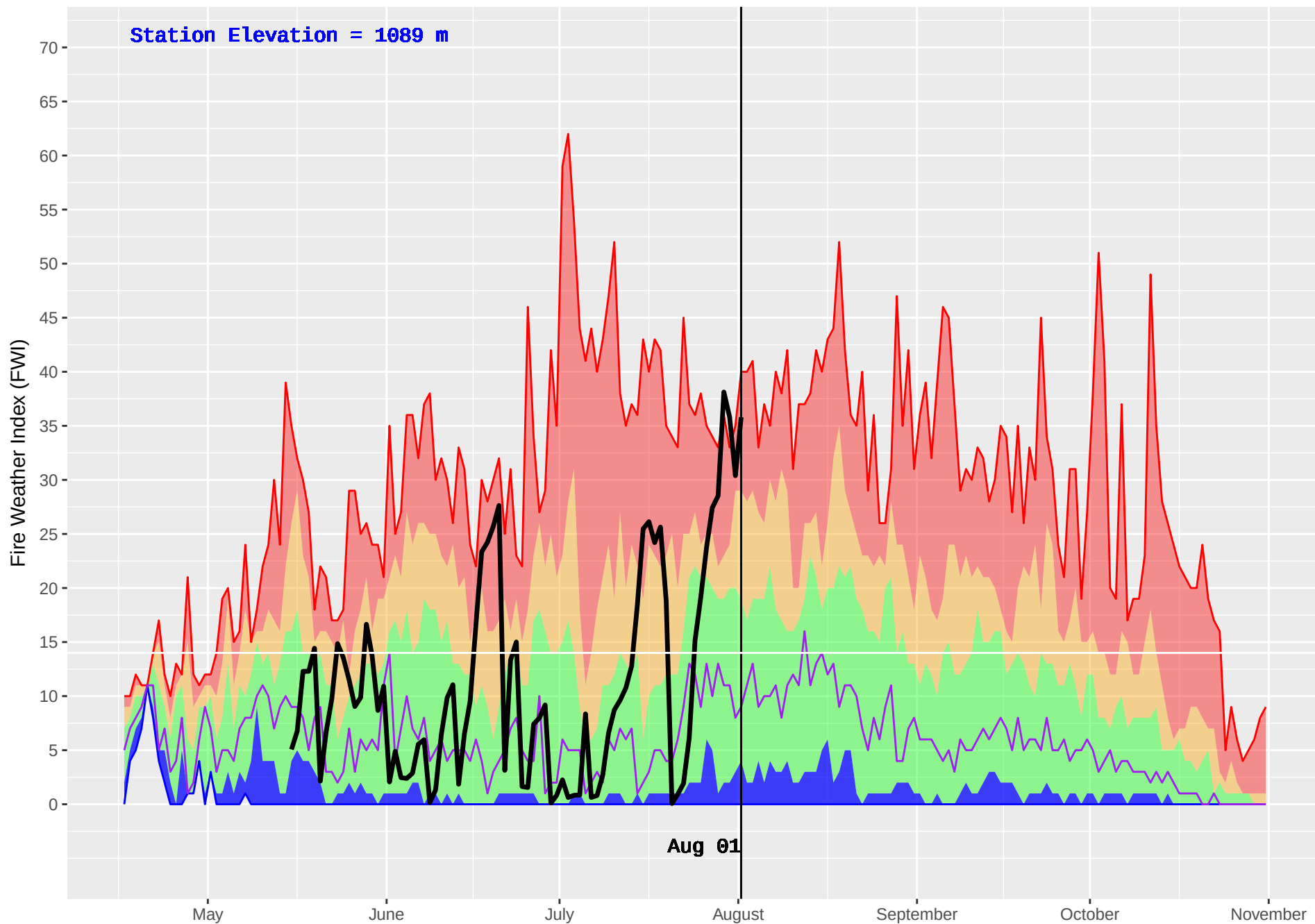
EAST OOTSA (170) : Historical (1986–2016) and Current (2018) Daily Fire Weather Index (FWI)
